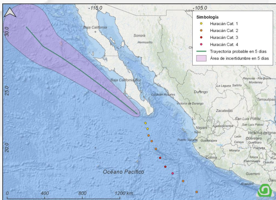
Trayectoria preliminar y pronóstico para cinco días del Huracán Genevieve. Fuente: NHC-NOAA Preliminary track and five-day forecast of Hurricane Genevieve. Source: NHC-NOAA
